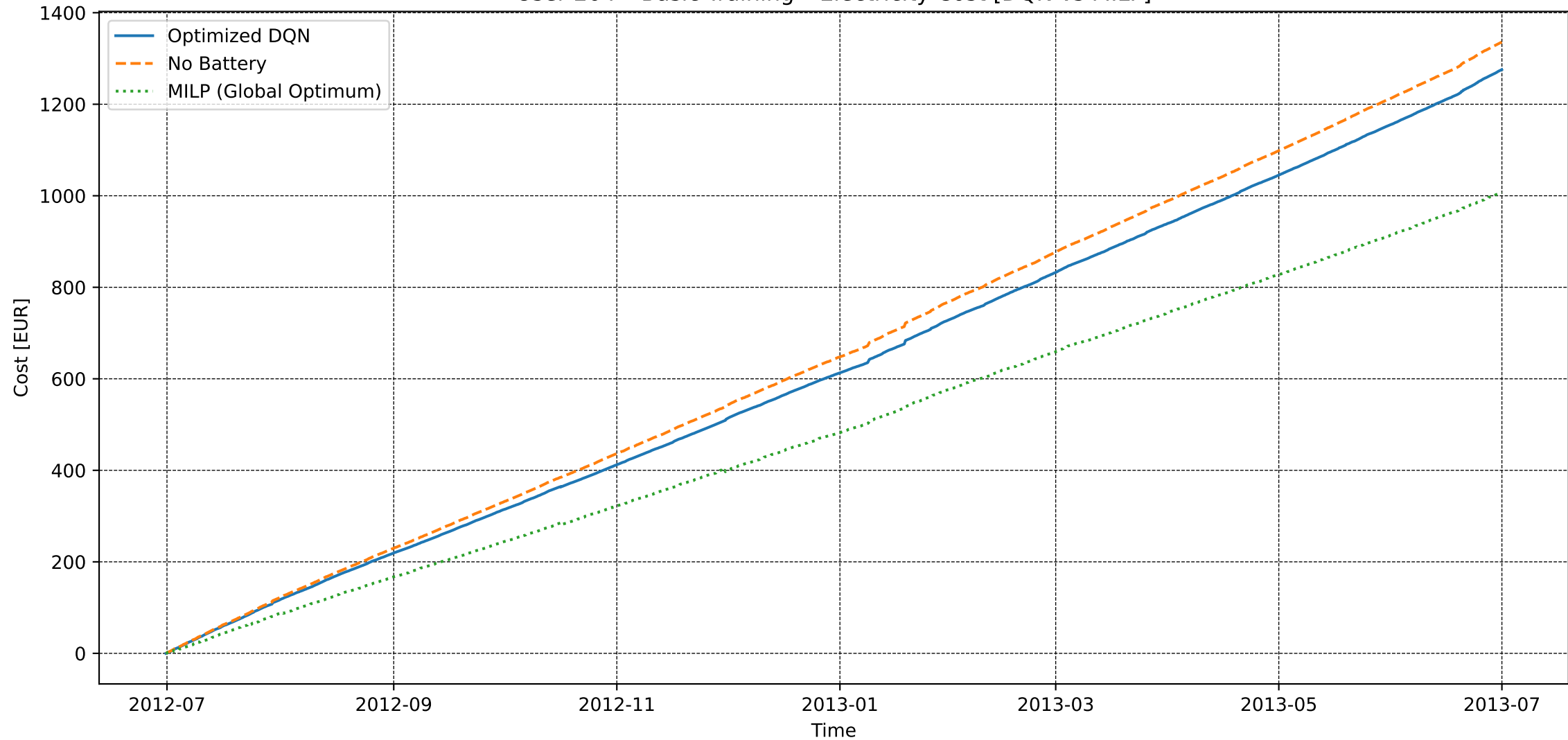
User 204 - Basic Training - Electricity Cost [DQN vs MILP]
